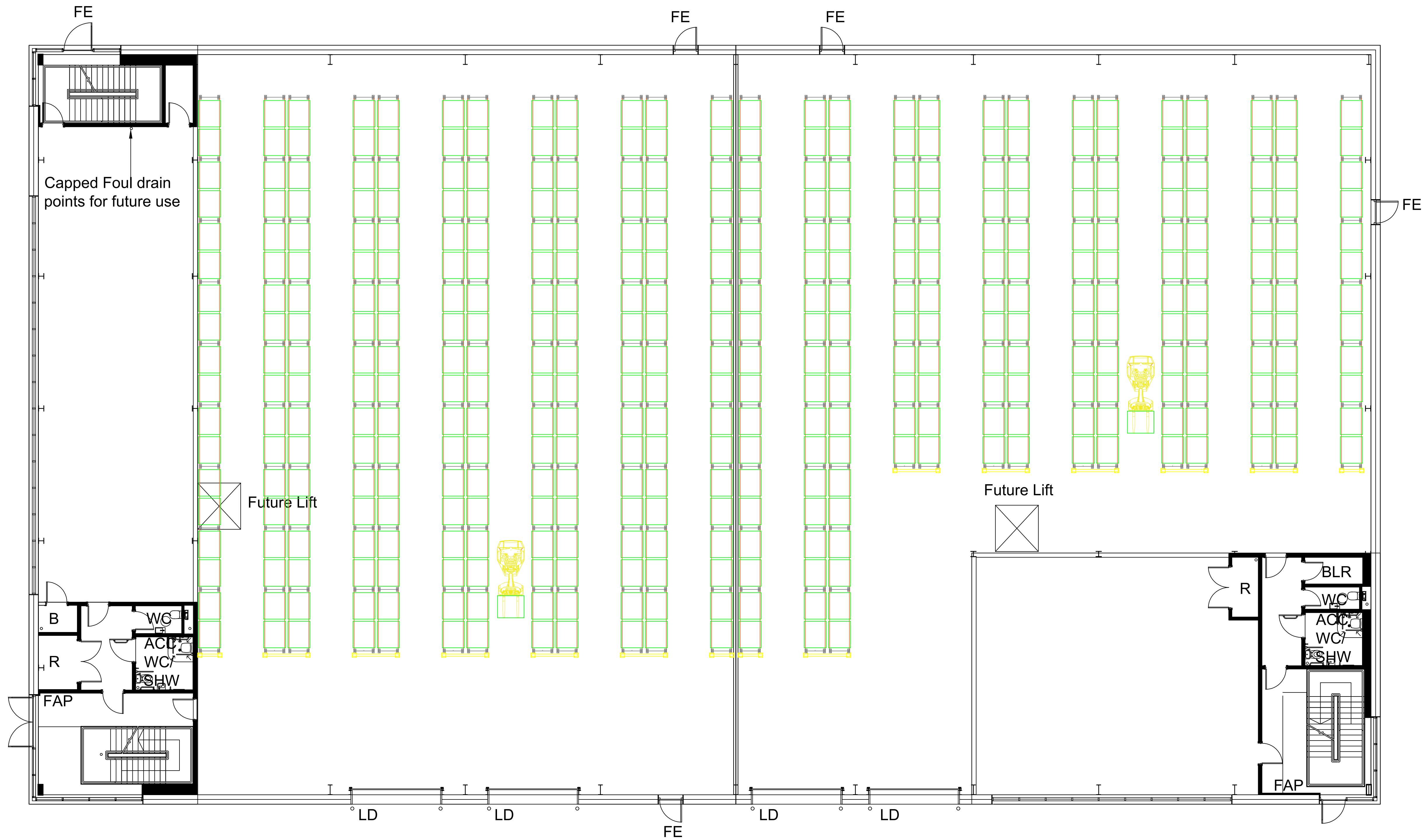
Unit 1 - (10m Eaves) 1296 UK Pallet Locations @ 1.5m
